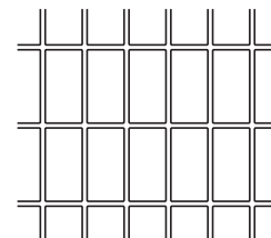
Stacked Bond Brick Size 197 x 99
